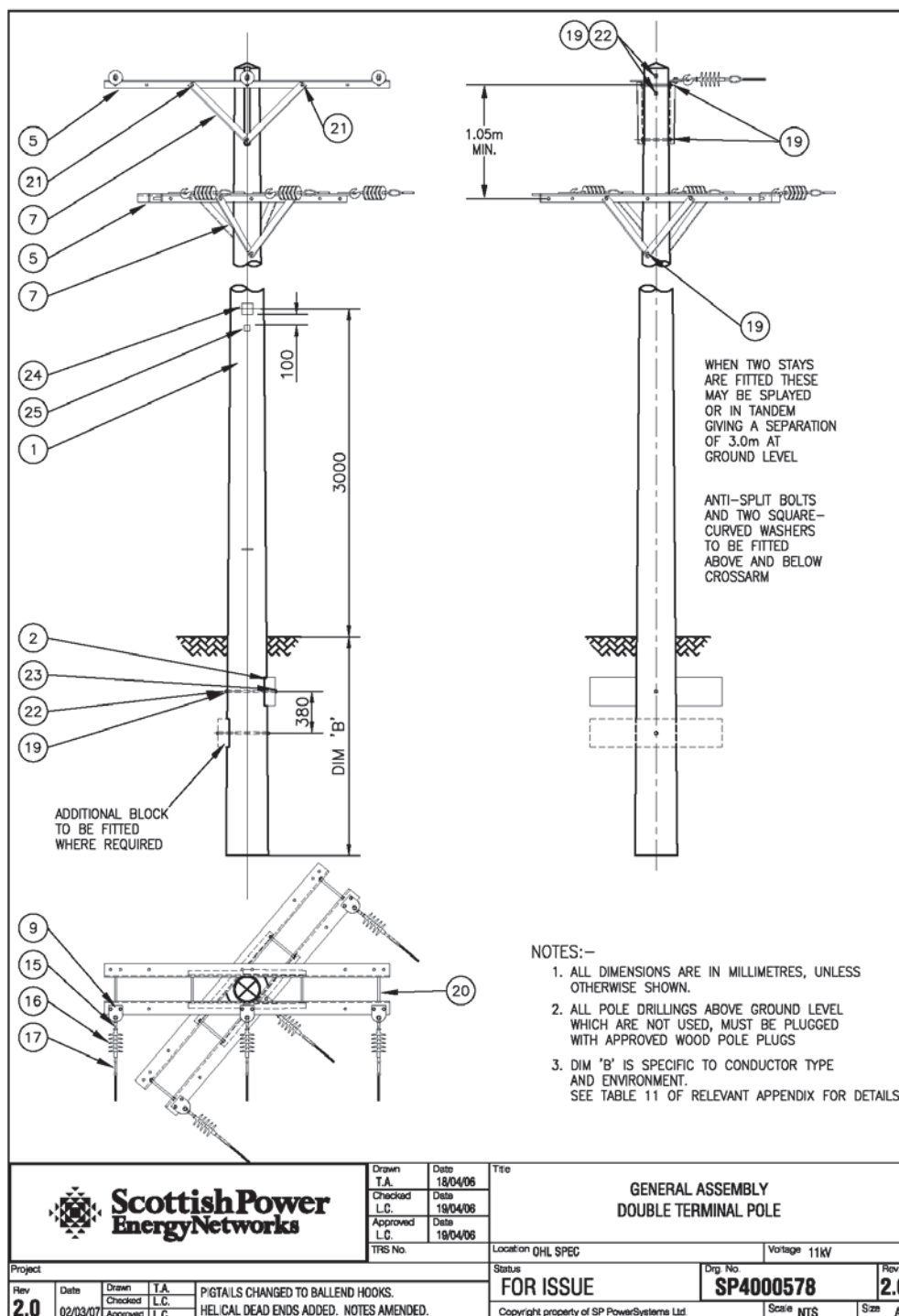
Figure 19 Single Pole Double Terminal (Drawing SP4000578)
